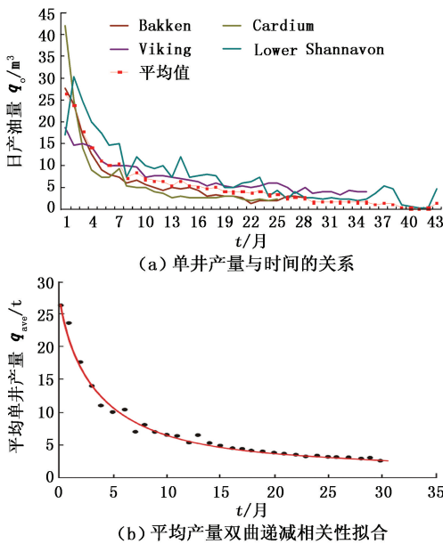
图 9 加拿大 4 个致密油区产量递减情况 Fig.9 Production decline of four tight oil zones in Canada
