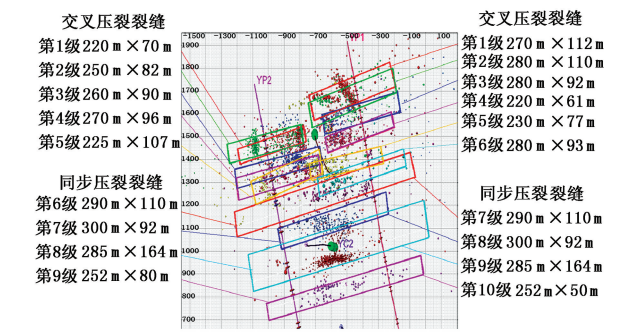
图2 YP水平井压裂裂缝微地震监测事件 Fig.2 Micro-seismic testing of fracture of YP horizontal wells
