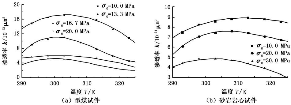
图 4 渗透率与温度关系 Fig. 4 Relationship between permeability and temperature
