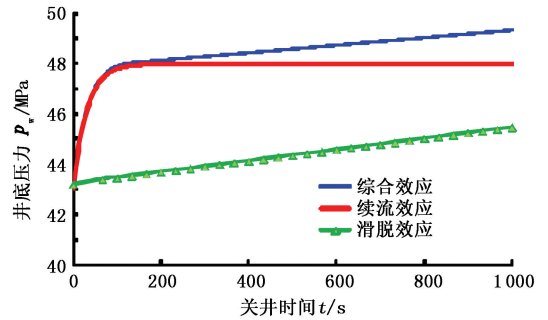
图 4 关井期间不同模型下的井底压力变化曲线 Fig. 4 Curves of bottom hole pressure change during well shut-in period
