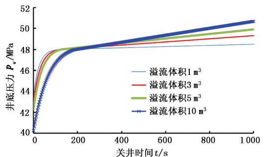
图 5 溢流体积对井底压力的影响 Fig. 5 Effect of pit gain on bottom hole pressure
