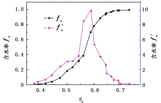
图 7 单一段塞注入微生物含水率导数曲线 Fig. 7 Moisture content derivative of single slug flooding
