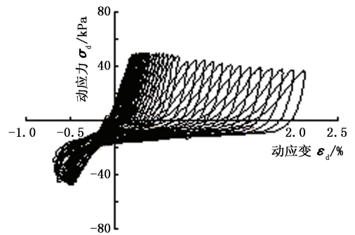
图 3 随振动次数的增加素土滞回圈的变化 Fig. 3 Change of plain soil hysteresis loops with increase of vibration times
