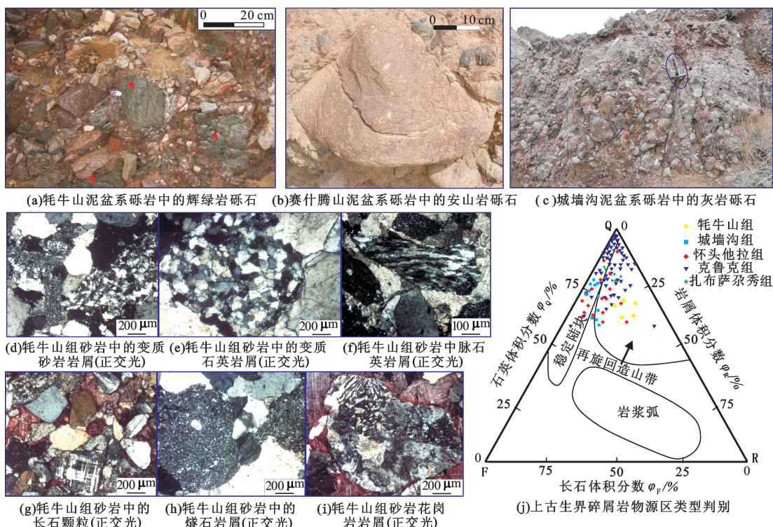
图 3 柴北缘泥盆系碎屑颗粒组成 Fig. 3 Devonian detrital composition in Northern Qaidam
